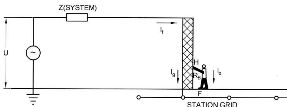
FIG. 4 EXPOSURE TO TOUCH VOLTAGE
