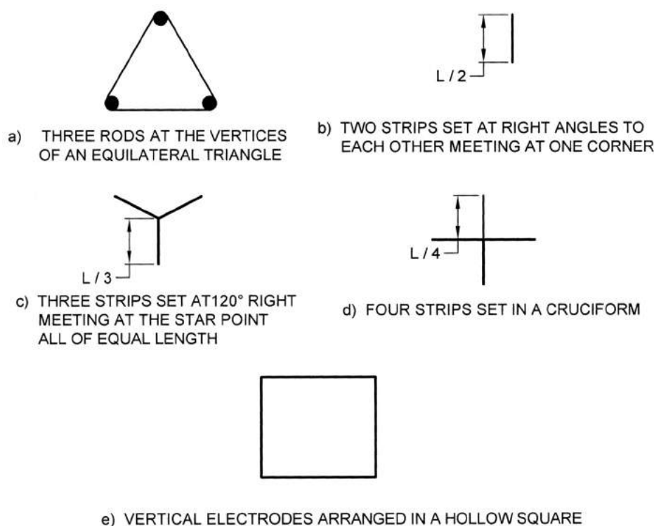
FIG. 24 MISCELLANEOUS ELECTRODE CONFIGURATIONS
