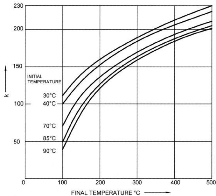
FIG. 28 k FACTORS FOR COPPER PROTECTIVE CONDUCTORS (see 17.2.2.1)
