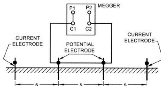
FIG. 48 TEST CONNECTION TO MEASURE THE SUM OF THE POTENTIAL ELECTRODE RESISTANCE
