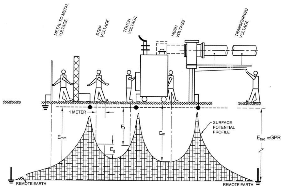
FIG. 9 BASIC SHOCK SITUATIONS
