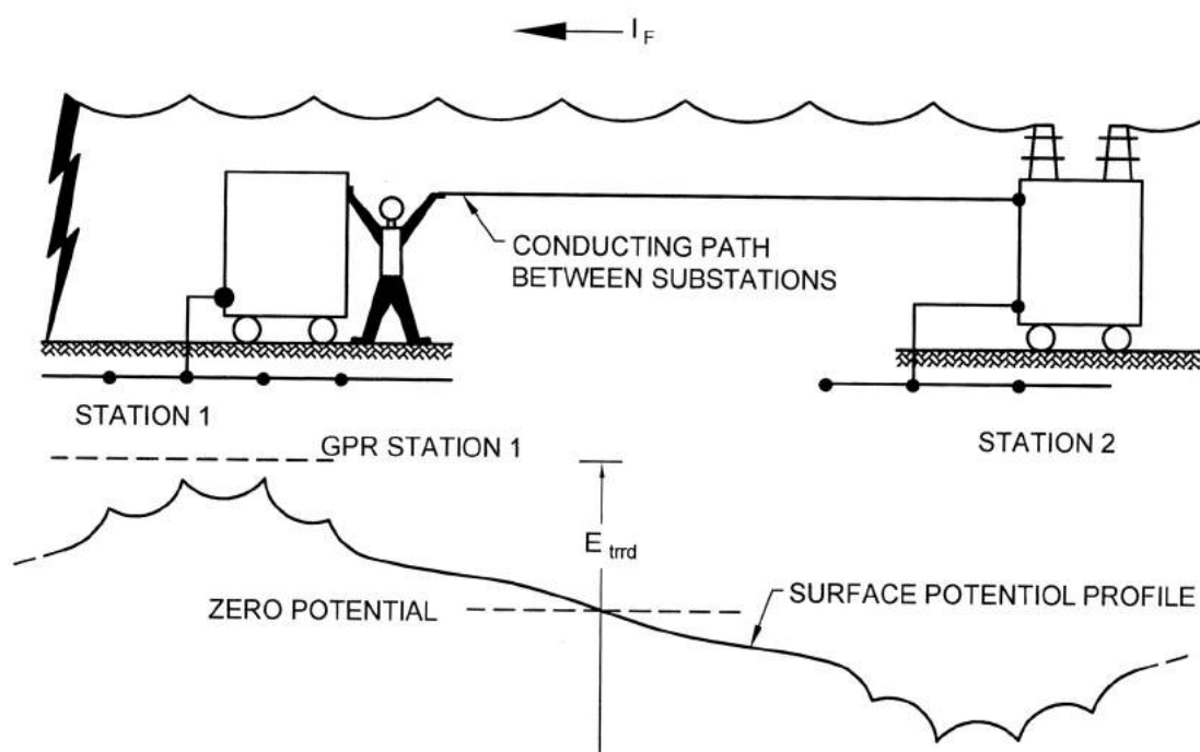
FIG. 10 TYPICAL SITUATION OF EXTENDED TRANSFERRED POTENTIAL
