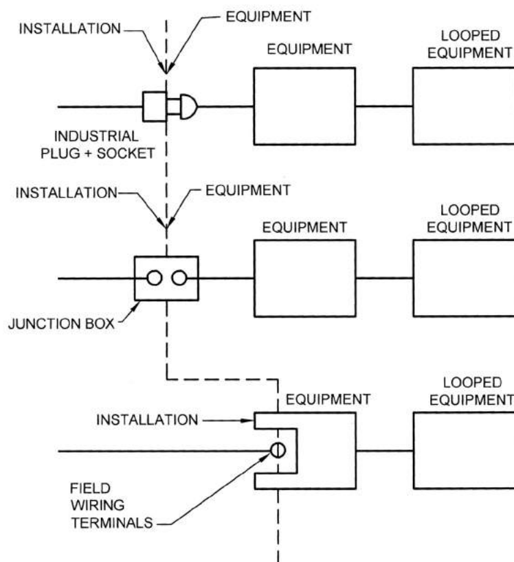
FIG. 55 EQUIPMENT-INSTALLATION BOUNDARIES
