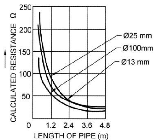
FIG. 21 EFFECT OF LENGTH OF PIPE ELECTRODE ON CALCULATED RESISTANCE FOR SOIL RESISTIVITY OF 100 \Omega \cdot \text{m} (ASSUMED UNIFORM)
